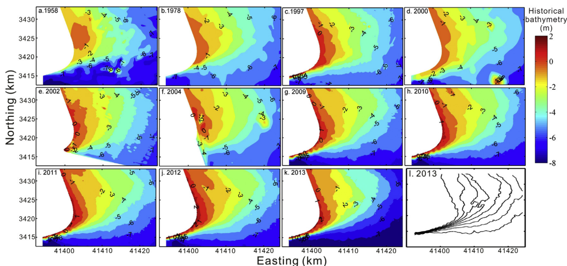
Fig. 2. Distribution of the Nanhui beach bathymetry in different years (a–k is bathymetric distribution in given year, and l is a contours drawn of bathymetric image in 2013).
