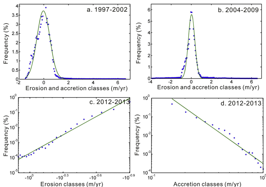
Fig. 5. Frequency of occurrence of erosion and accretion events in different intervals in different years.
