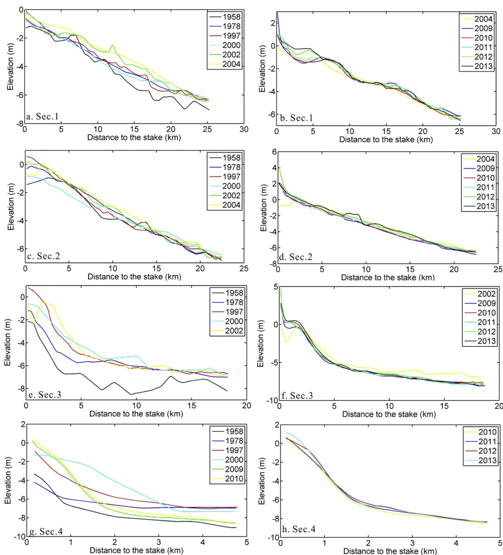
Fig. 6. Beach profile changes of the different parts along Nanhui (the distance to 1958 0 m shoreline stake).
