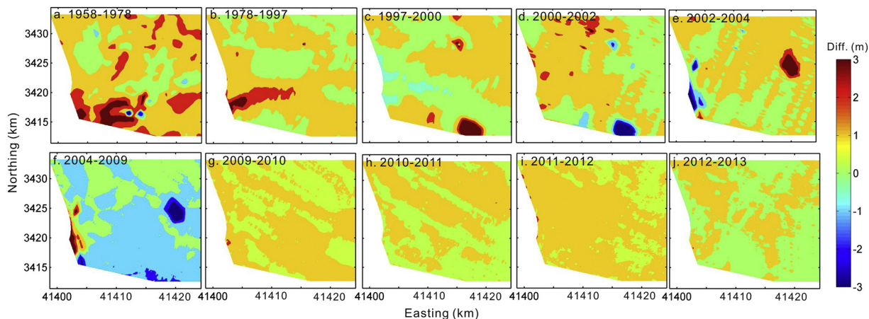
Fig. 4. Changes of accretion and erosion (depth of later time minus that of the previous time) in the Nanhui beach in different years.
